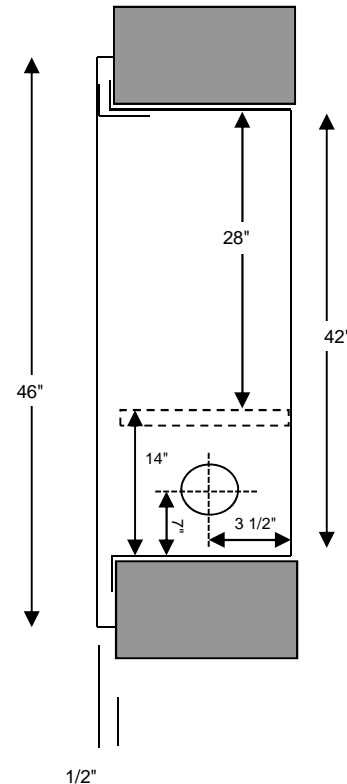
SIDE
